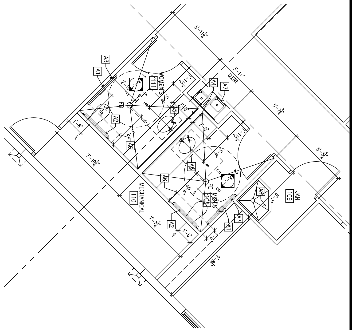
4 ENLARGED RESTROOM PLAN A2.0 1/4"=1'-0"
