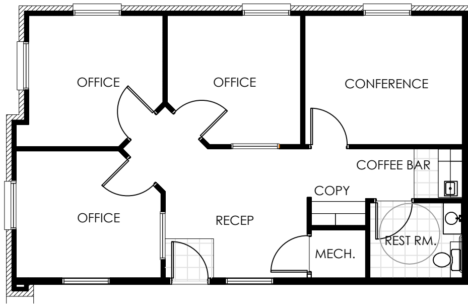
FLOOR PLAN
