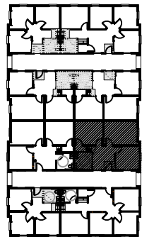
KEY PLAN - Building "L"
