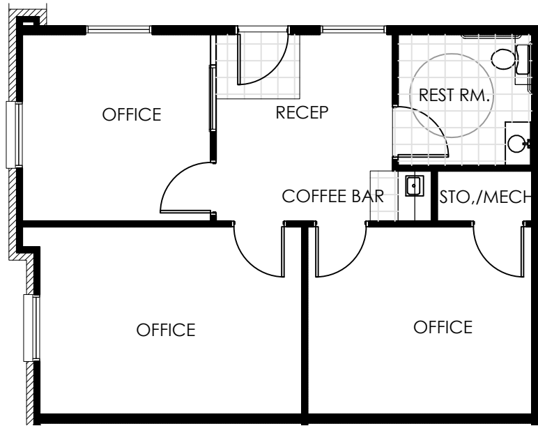
FLOOR PLAN
