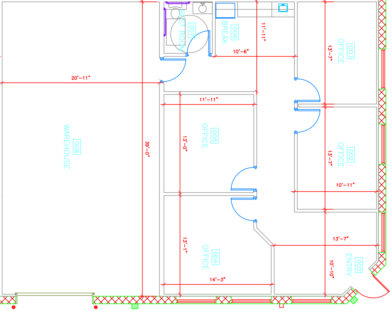
1 1/8" = 1'-0" Floor Plan Suite 410 2,054 sq. ft.
