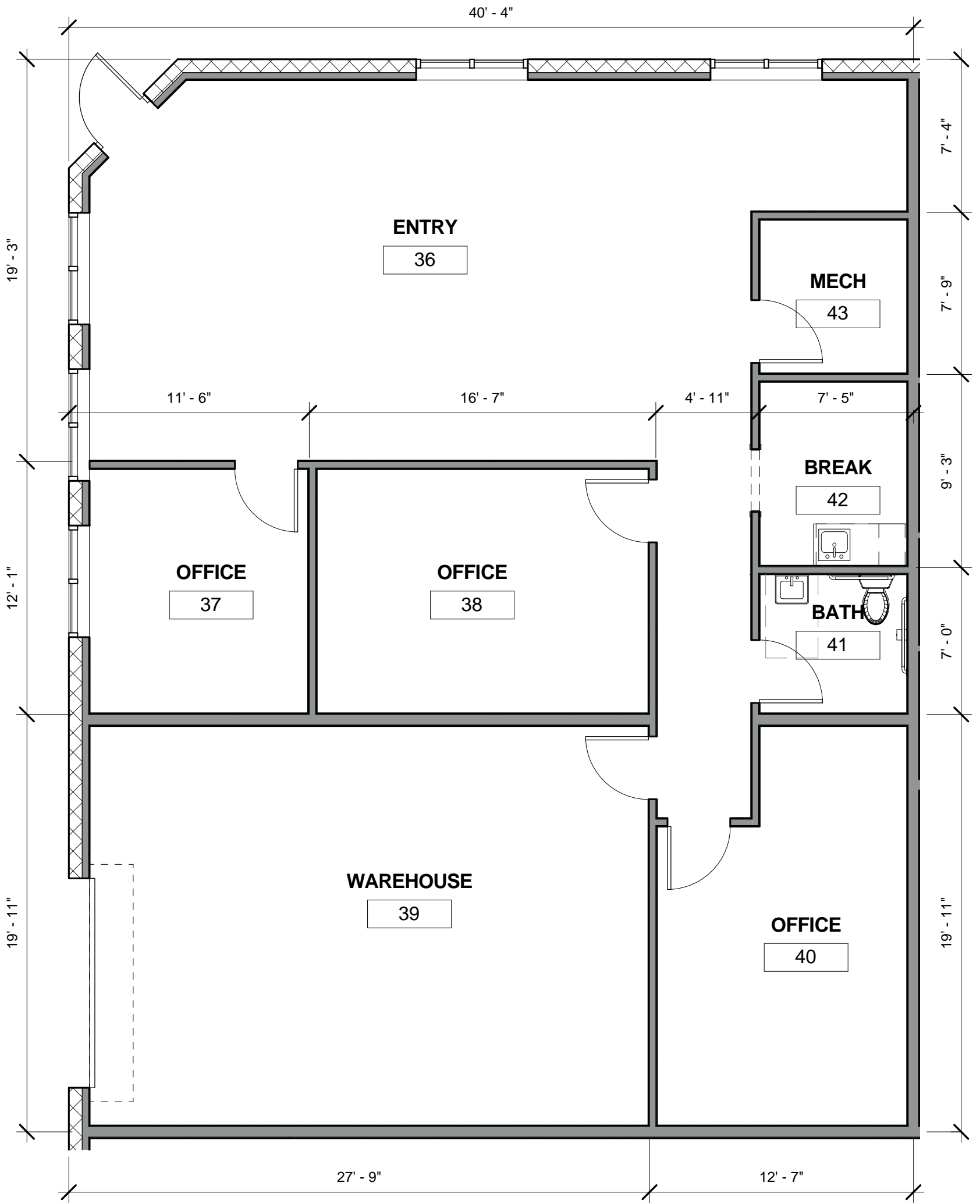
① SUITE 200 3/16" = 1'-0"
